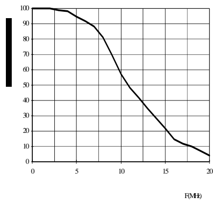
Fig. 2 Typical square-wave response curve
