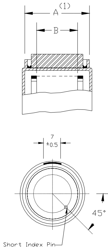
FRONT VIEW XQ2172/02 Figure 2
