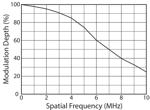
Figure 4. Typical Square-wave response curve for XQ1585A camera tube
