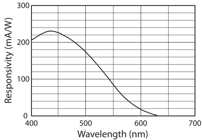
Figure 3. Typical spectral response curve for XQ1585A camera tube
