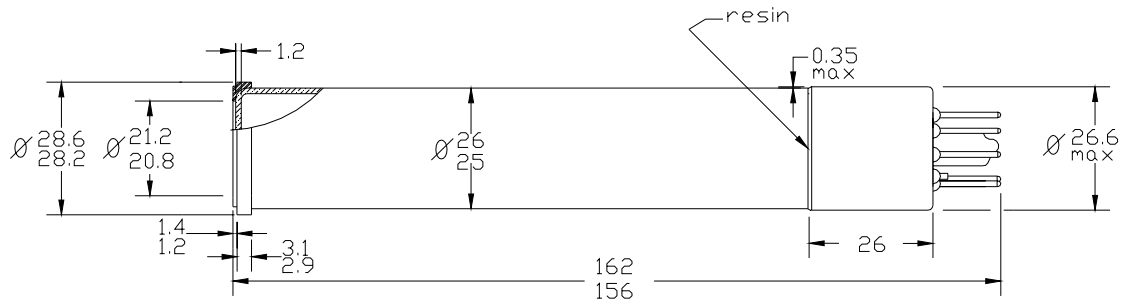
Figure 1. Mechanical data for XQ1585A camera tube
