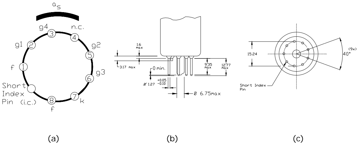
Figure 2. Mechanical data for XQ1585A camera tube
