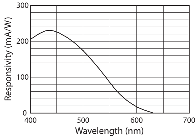
Figure 3. Typical spectral response curve for XQ1570A camera tube
