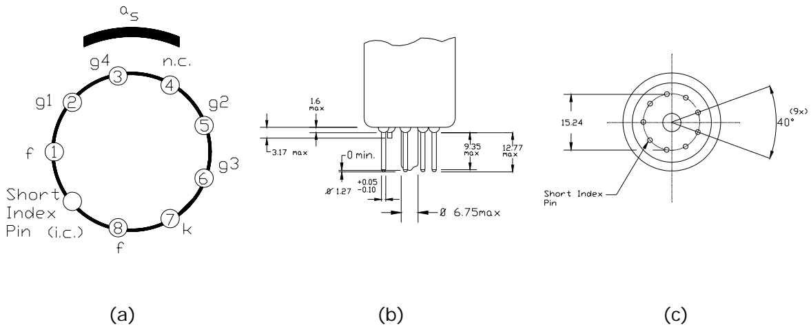
Figure 2. Mechanical data for XQ1570A camera tube
