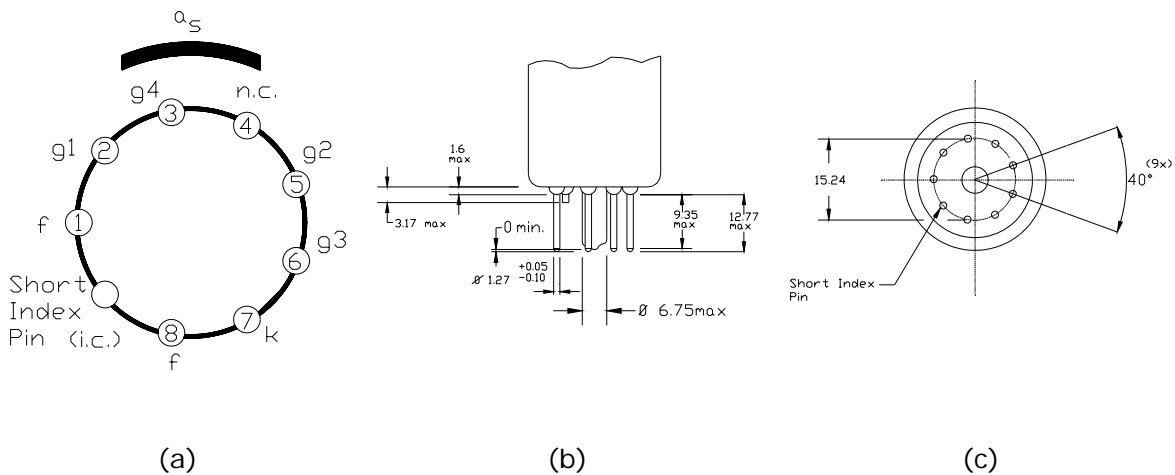
Figure 2. Mechanical data for XQ1565A camera tube
