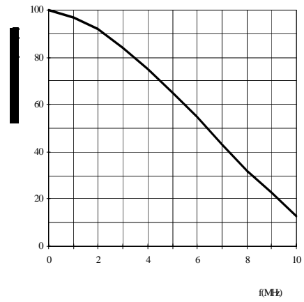
Fig. 2 Typical square-wave response curve.
